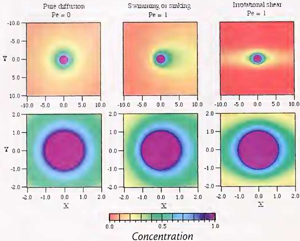
Figure 6. Concentration distributions of a hypothetical chemical signal molecule uniformly released from the surfaces of microscopic point sources (purple circles) in three different flow regimes: stagnant water (pure diffusion, no advective transport); uniform flow ( i.e. , cell swimming or sinking in stagnant water; the cell is moving from right to left so flow is from left to right); and laminar shear flow (uniaxial extensional flow), where the third dimension can be visualized by rotation about the x -axis. The Peclet number ( Pe ) is a measure of advective transport relative to molecular diffusion (where Pe = LU/D_m ; L = characteristic length scale, U = characteristic velocity scale, and D_m = coefficient of molecular diffusion). The upper panel illustrates the concentration field at distances up to 10 cell radii from the center of the cell. The lower panel is a "blow-up" of the concentration field near the cell surface, up to a distance of two radii from the center of the cell. In the absence of fluid motion a diffusive boundary layer extends to about nine cell radii from the cell surface. Uniform and shear flows distort the boundary layer and steepen the concentration gradient in certain regions. Because transport via diffusion is dominant in the thinnest regions of the boundary layer, cells in uniform or shear flow will experience enhanced rates of chemical signal release compared to nonmotile cells in stagnant water. This illustration was provided as a courtesy by L. Karp-Boss, and methods used in calculating concentration distributions appeared in Karp-Boss et al. (1996).
